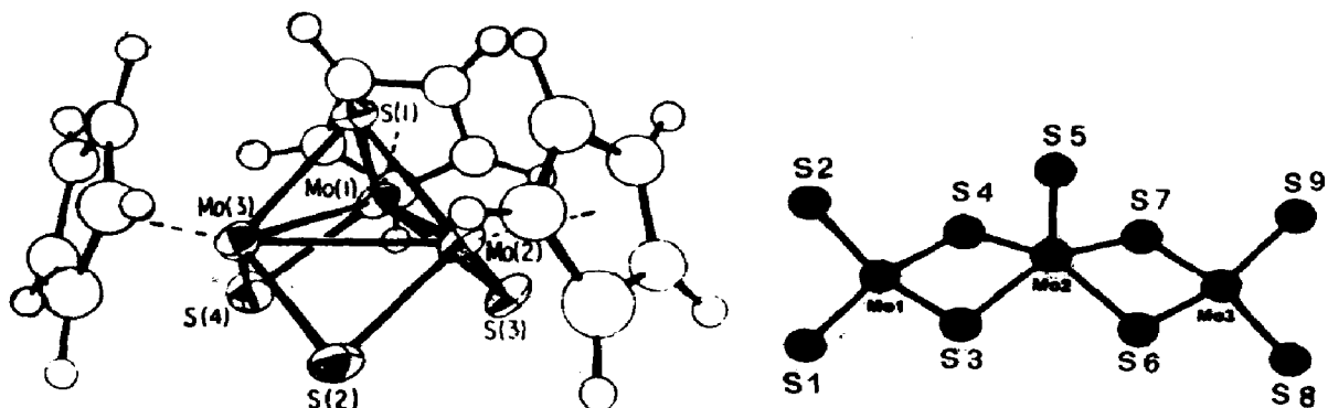
Fig. 65. Perspective view of [\text{Mo}_3\text{S}_4(\text{C}_5\text{H}_5)_3]^+ . Average distances for core: Mo–Mo 2.81 Å, Mo– \mu_3 -S 2.31 Å, Mo– \mu_2 -S 2.29 Å (from ref. 138).
