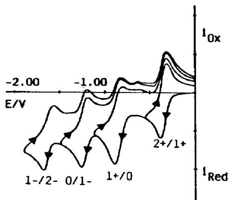
Fig. 56. Cyclic voltammetric response recorded for an acetonitrile solution of [\text{Ni}_3\text{S}_2(\text{PET}_3)_6]^{2+} . Potential values vs. S.C.E.
