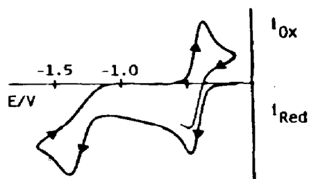
Fig. 7. Cyclic voltammetric behaviour of \text{Fe}_3(\text{CO})_9\text{S}_2 in benzonitrile solution. Potential values vs. Ag/AgCl.
