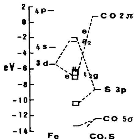
Fig. 3. MO diagram for \text{Fe}_3(\text{CO})_9(\text{S})(\text{CO}) .
