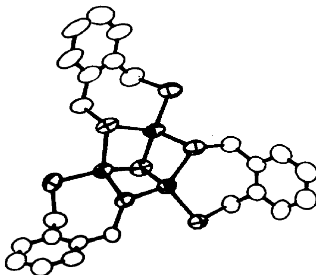
Fig. 4. Crystal structure of the dianion [\text{Fe}_3\text{S}(1,2-(\text{SCH}_2)_2\text{C}_6\text{H}_4)_3]^{2-} (from ref. 17).
