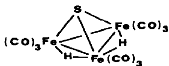
Fig. 1. Proposed structure of the complex \text{H}_2\text{Fe}_3(\text{CO})_9(\mu_3\text{-S}) .
