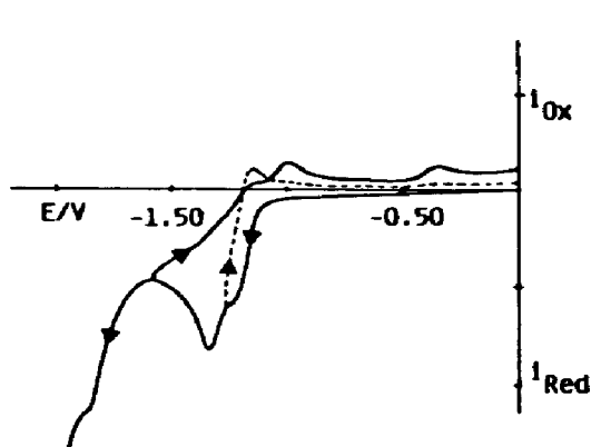
Fig. 56. Cyclic voltammetric response recorded for an acetonitrile solution of [\text{Ni}_3\text{S}_2(\text{PET}_3)_6]^{2+} . Potential values vs. S.C.E.
